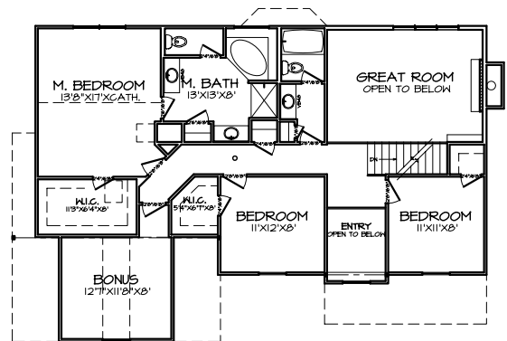
SECOND FLOOR PLAN A-5
