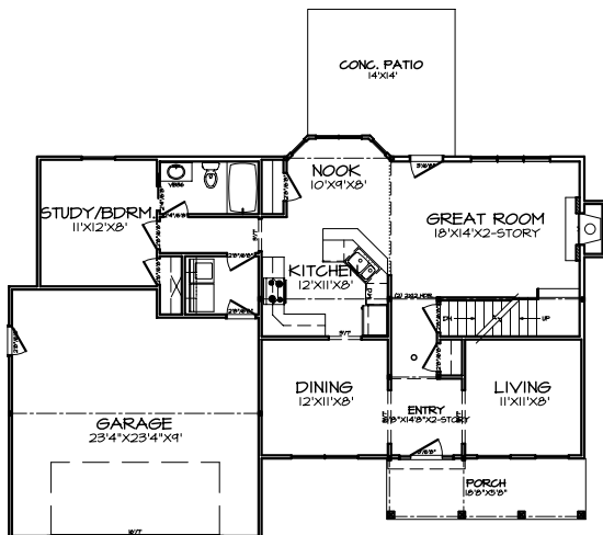
FIRST FLOOR PLAN A-4
