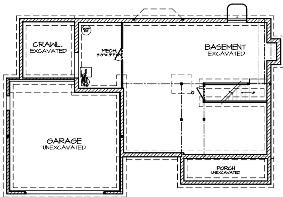
FOUNDATION PLAN A-3
